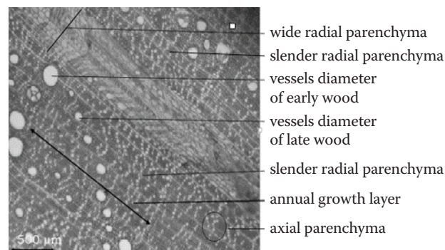
Fig. 3. Transversal plane of Quercus ilex Linnaeus
