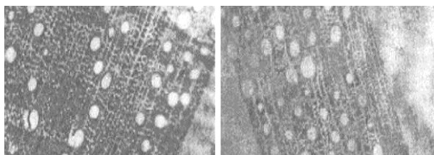
Fig. 4. Variation in the disposition of the pores of Quercus ilex Linnaeus in internal (a) and external (b) area
