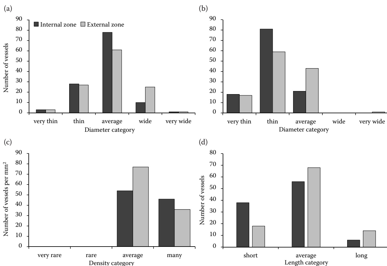
Fig. 5. Histograms of wood characteristics of the vessels: diameter in early wood (a), diameter in latewood (b), density (c), length (d)
