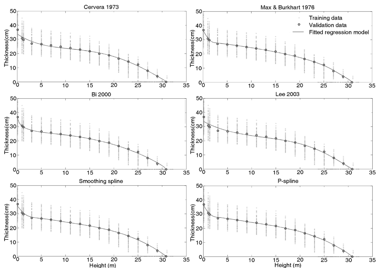
Fig. 2. Selected taper models based on 84 stems and the validation stem fitted by the model
