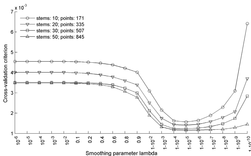
Fig. 1. Cross-validation values in dependence on smoothing parameter for smoothing spline. Separate lines show the development of CV criterion for different density of training points expressed as the number of trees
