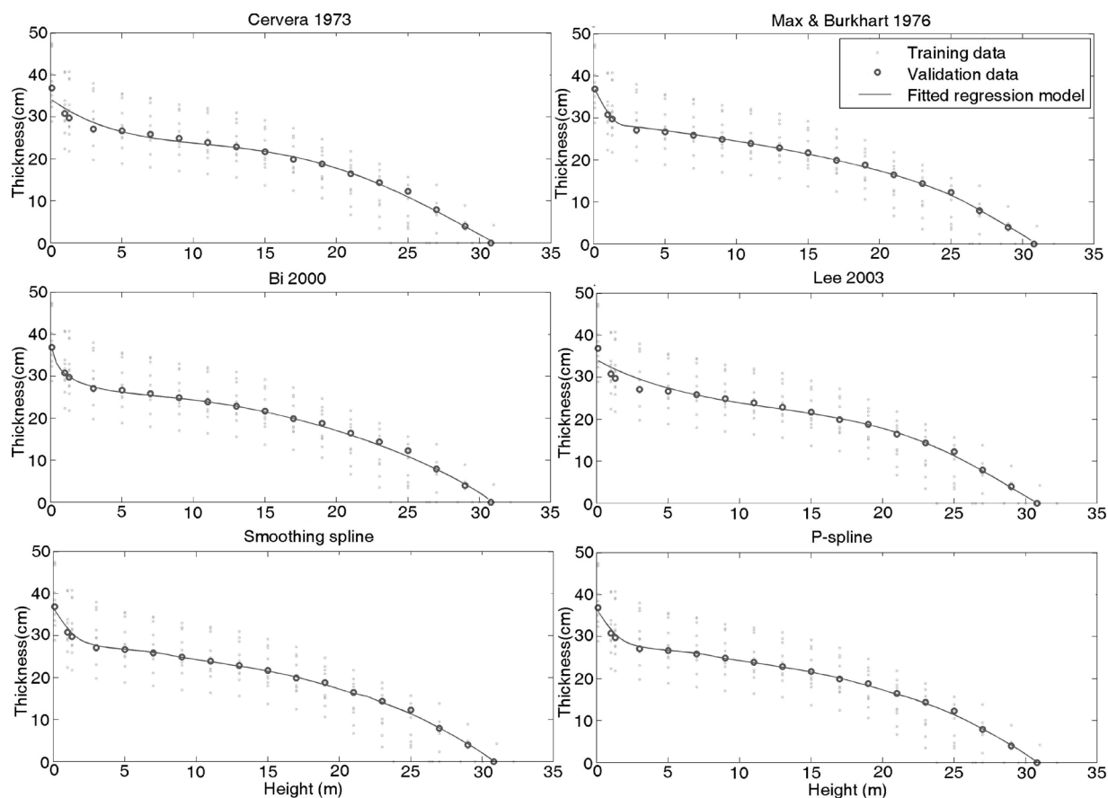
Fig. 3. Selected taper models based on 10 stems and the validation stem fitted by the model
