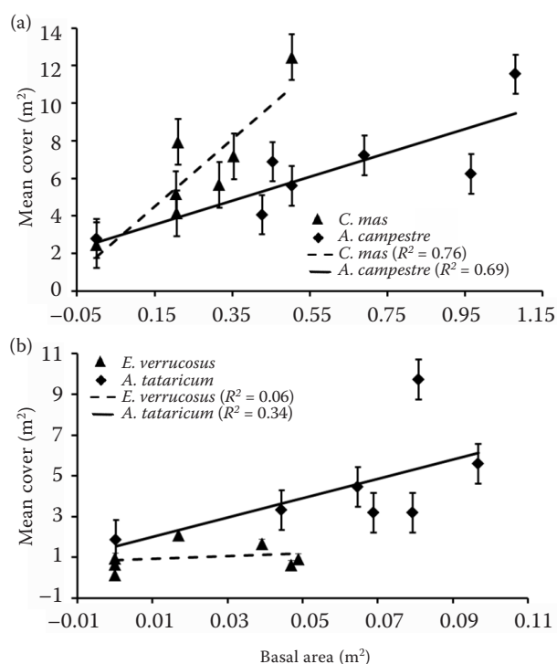
Fig. 2. Regression models relating the mean cover of dominant woody species and their basal area ( \pm S.E.) by the understorey layer during 1972–2007 in the sample site R^2 – coefficient of determination of linear regression
