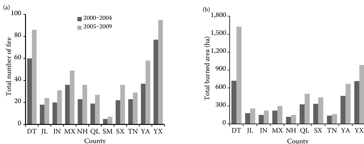
Fig. 2. Fire number (a) and burned areas (b) in two study periods
