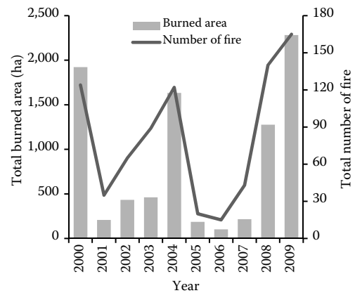
Fig. 5. Distribution of forest fires and burn areas from 2000 to 2009
