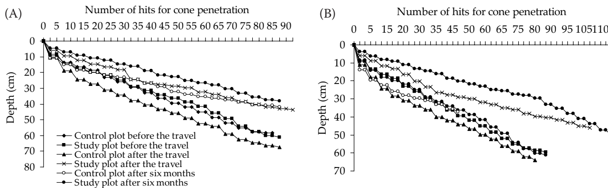
Fig. 3. Penetration curves on study plot No. 4, Rudice, Zetor 7245 universal wheeled tractor, three sets of measurements – (A) the first set and (B) the second set of measurement
