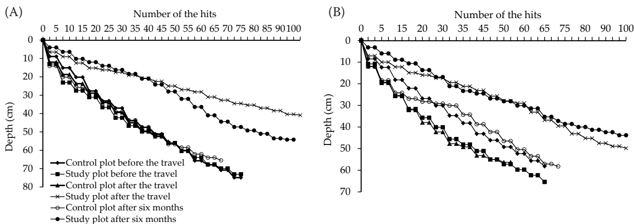
Fig. 1. Penetration curves on study plot No. 2, Babice nad Svitavou, Zetor 7245 universal wheeled tractor, three sets of measurements – (A) the first set and (B) the second set of measurement
