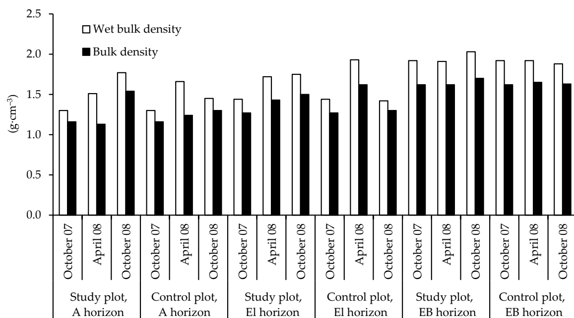
Fig. 5. Wet bulk density and bulk density for the particular soil horizons of study plot No. 3 and the control plot, Rudice, PONSSE ERGO harvester and GREMO 950 forwarder
