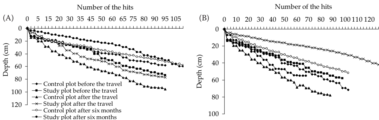
Fig. 2. Penetration curves on study plot No. 3, Rudice, PONSSE ERGO harvester and GREMO 950 forwarder, three sets of measurements – (A) the first set and (B) the second set of measurement
