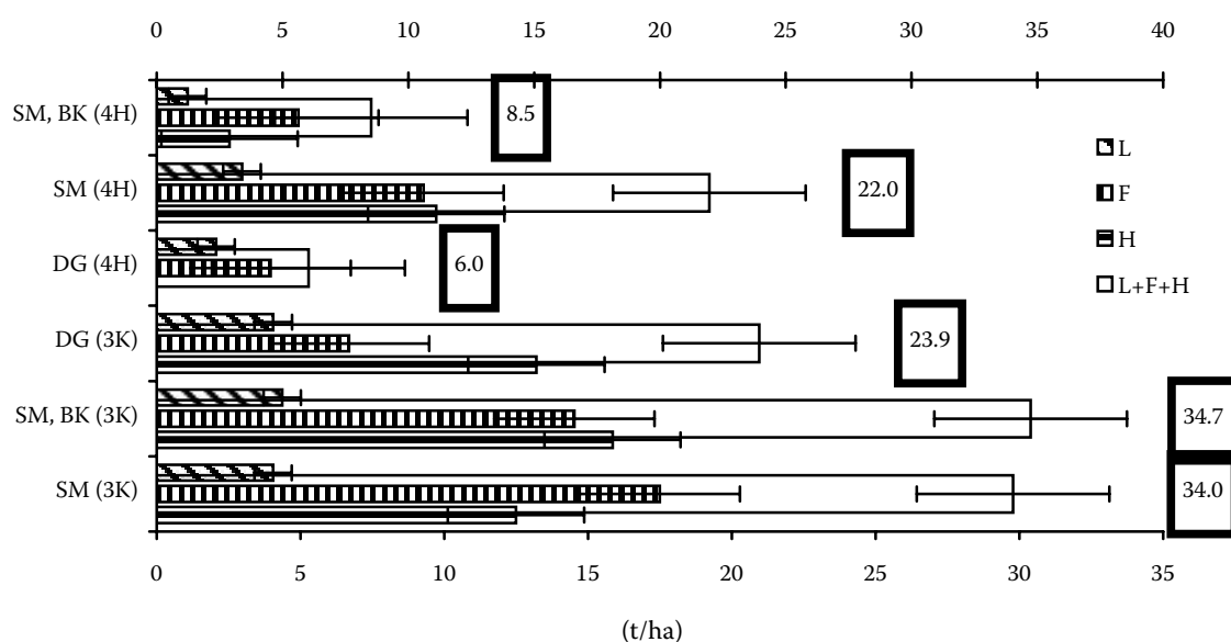
Fig. 4. Carbon reserves in forest floor in different forest stands (I – confidence interval [0.95], lower x-axis – reserves of the carbon separate layers [L, F, H] of forest floor, upper x-axis – total accumulation of carbon in surface humus [L+F+H])
