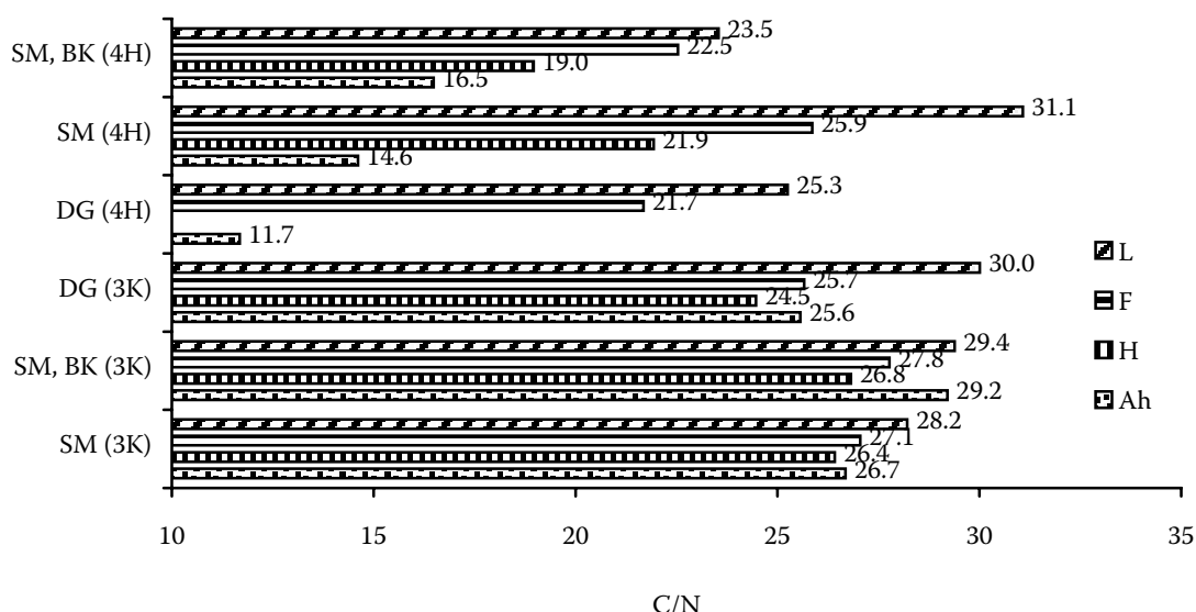
Fig. 6. C/N ratio in forest floor in different forest stands (value of a mixed sample – 10 samplings of particular layers [L, F, H]; 5 samplings of a particular horizon Ah and a stand)
