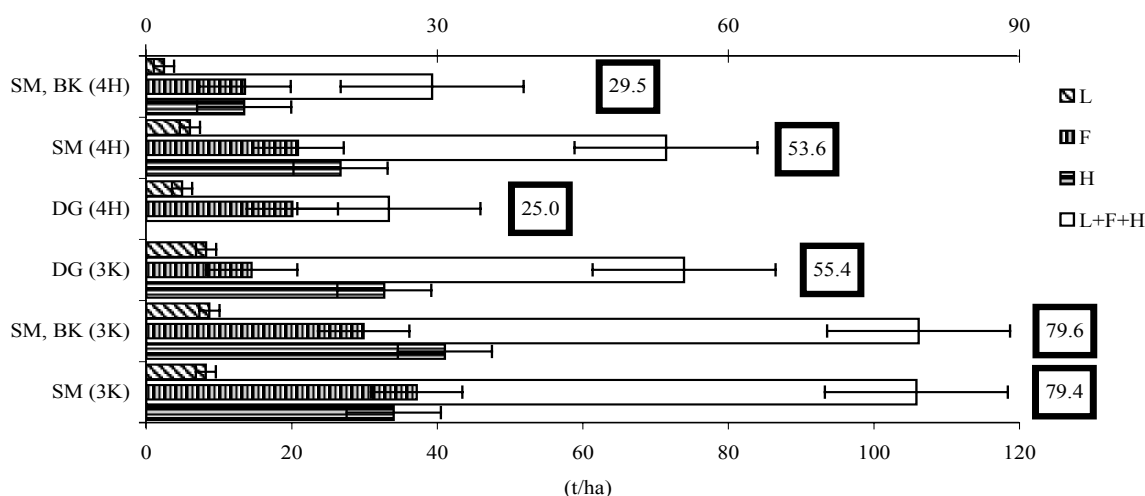
Fig. 1. Reserves of forest floor in different forest stands (I – confidence interval [0.95], lower x-axis – reserves of the separate layers [L, F, H] of forest floor, upper x-axis – total accumulation of surface humus [L+F+H])
