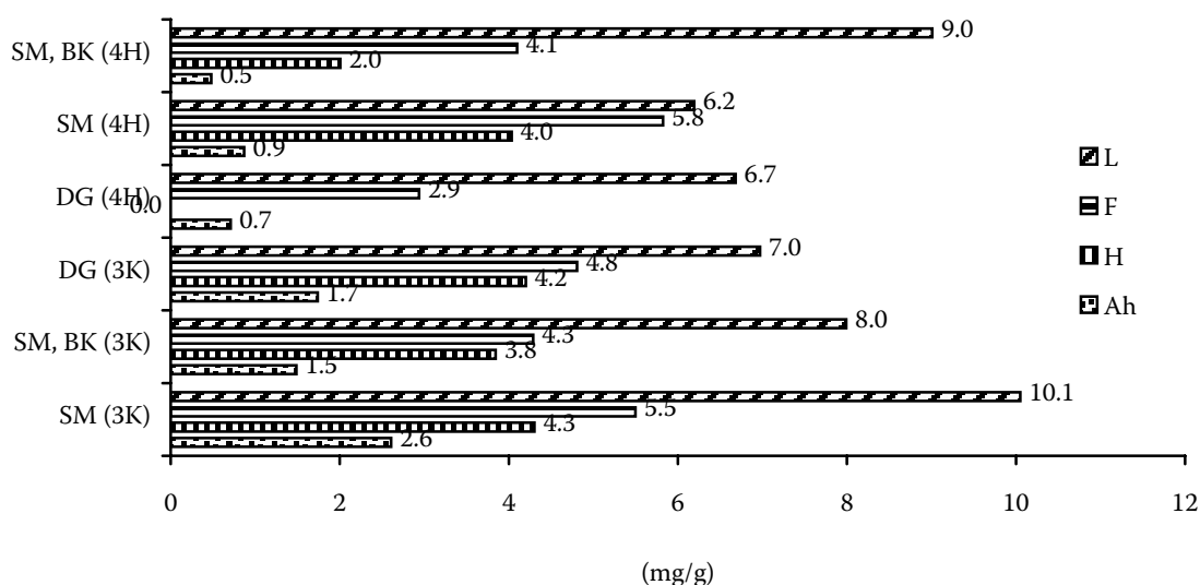
Fig. 7. The content of dissolved organic carbon (DOC) in forest floor in different forest stands (value of a mixed sample – 10 samplings of particular layers [L, F, H]; 5 samplings of a particular horizon Ah and a stand)
