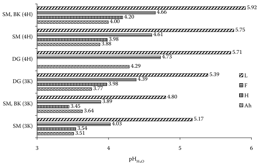
Fig. 2. Distribution of pH H 2 O in layers of forest floor and organo-mineral horizon in different forest stands (value of a mixed sample – 10 samplings of particular layers [L, F, H]; 5 samplings of a particular horizon Ah and a stand)
