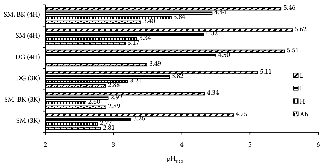
Fig. 3. Distribution of pH_{KCl} in layers of forest floor and organo-mineral horizon in different forest stands (value of a mixed sample – 10 samplings of particular layers [L, F, H]; 5 samplings of a particular horizon Ah and a stand)
