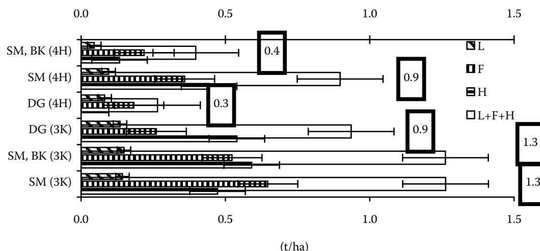
Fig. 5. Nitrogen reserves in forest floor in different forest stands (I – confidence interval [0.95], lower x -axis – reserves of the nitrogen separate layers [L, F, H] of forest floor, upper x -axis – total accumulation of nitrogen in surface humus [L+F+H])
