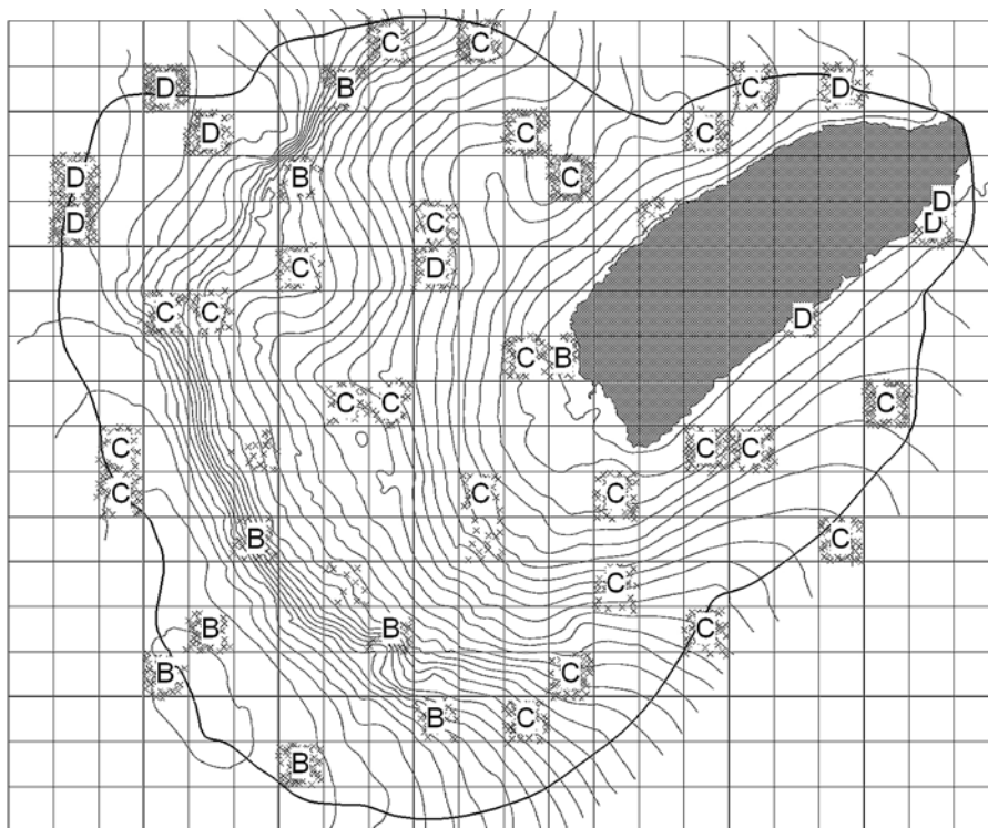
Fig. 2. Catchment of the Plešné jezero Lake with sample squares (50 m × 50 m in size) classified according to Clark-Evans' statistics: A – CE < 0.8 ; B – 0.8 \leq CE < 1.2 ; C – 1.2 \leq CE < 1.4 ; D – CE \geq 1.4 . The position of each tree in the sample square is indicated by a small cross. Terrain elevation is indicated by contour lines with 10 m interval
