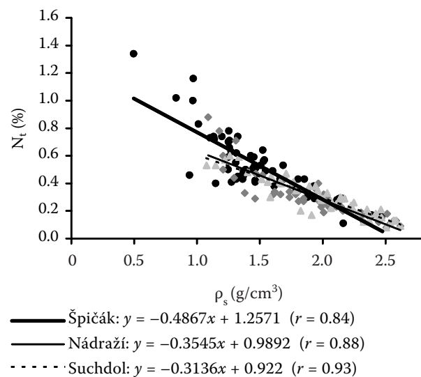
Fig. 5. Linear regression of \rho_s and N_t
