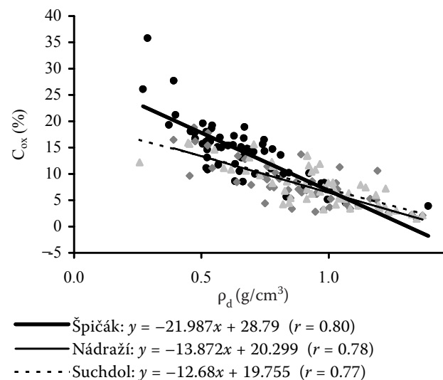
Fig. 2. Linear regression of \rho_d and C_{ox}
