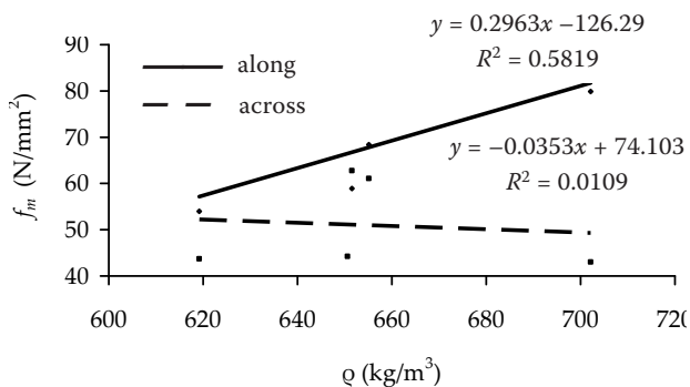
Fig. 11. Dependence of bending strength on the sheet density in combined plywoods
