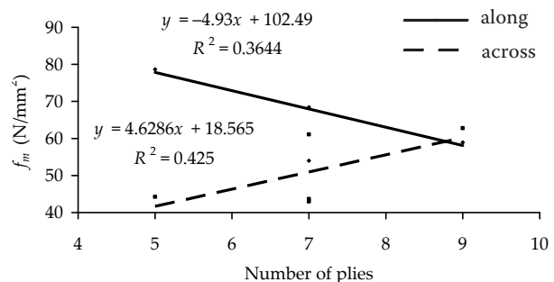
Fig. 14. Dependence of bending strength on the number of sheet plies in combined plywoods
