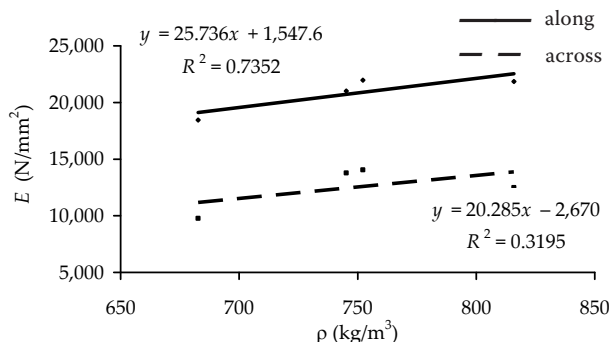
Fig. 19. Dependence of MOE on the sheet density in all-beech plywoods
