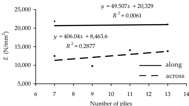
Fig. 22. Dependence of MOE on the number of sheet plies in all-beech plywoods
