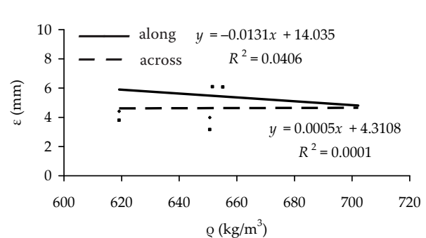
Fig. 12. Dependence of relative deformation on the sheet density in combined plywoods
