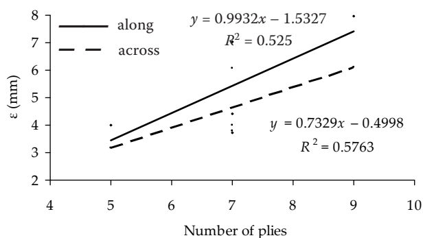
Fig. 15. Dependence of relative deformation on the number of sheet plies in combined plywoods
