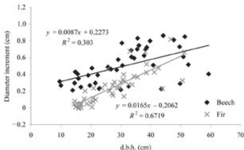
Fig. 6. Relationship between the total annual diameter increment of silver fir and beech and tree diameter in 2001
