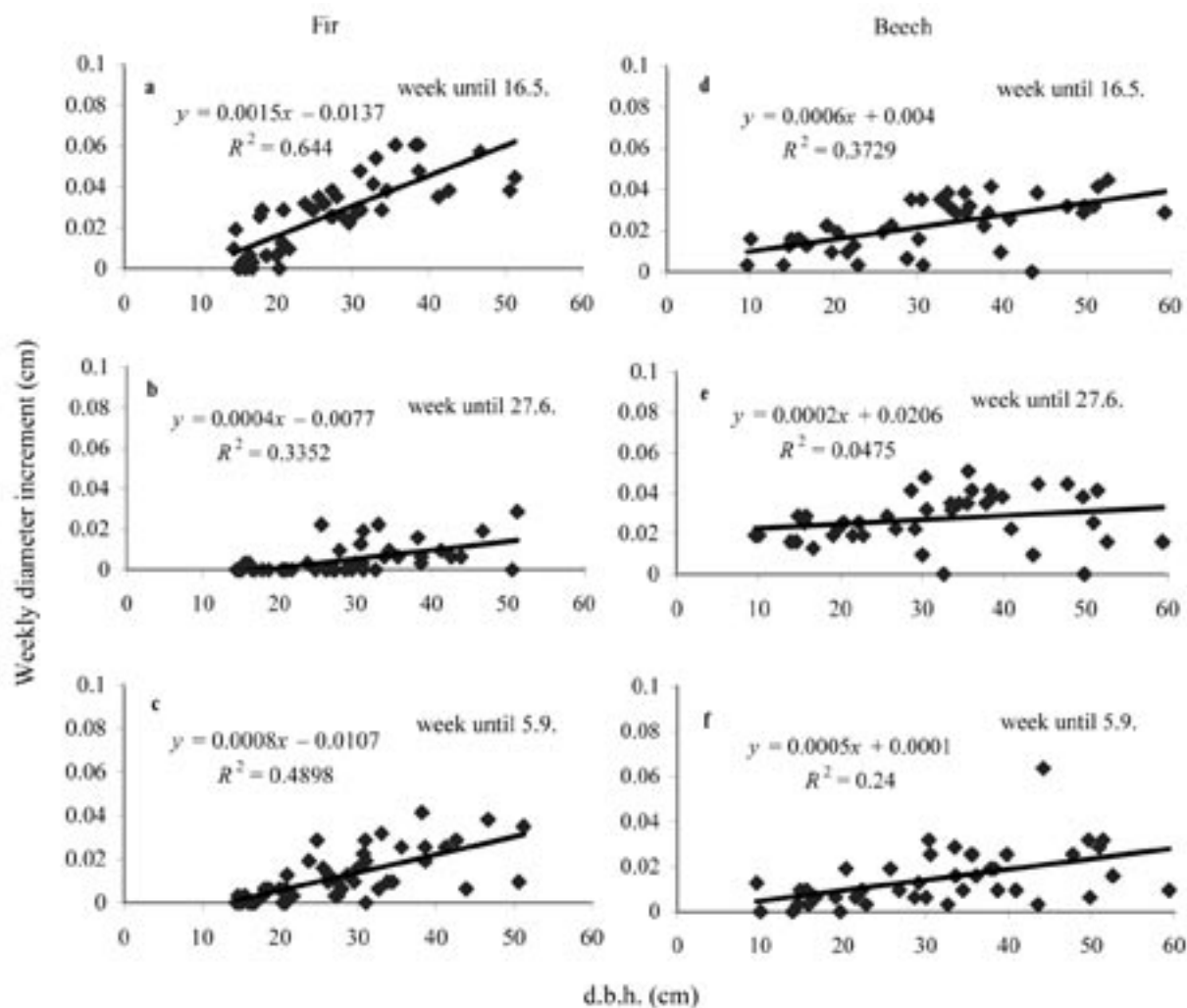
Fig. 5. Relationships between the diameter increment of silver and beech and diameter of trees in weeks until 16. 5. (a, d), 27. 6. (b, e) and 5. 9. 2001 (c, f)
