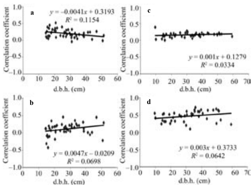
Fig. 7. Correlation between the magnitude of the current increment of all trees in particular weeks and weekly climatic data (a, c – precipitation, b, d – temperature)
