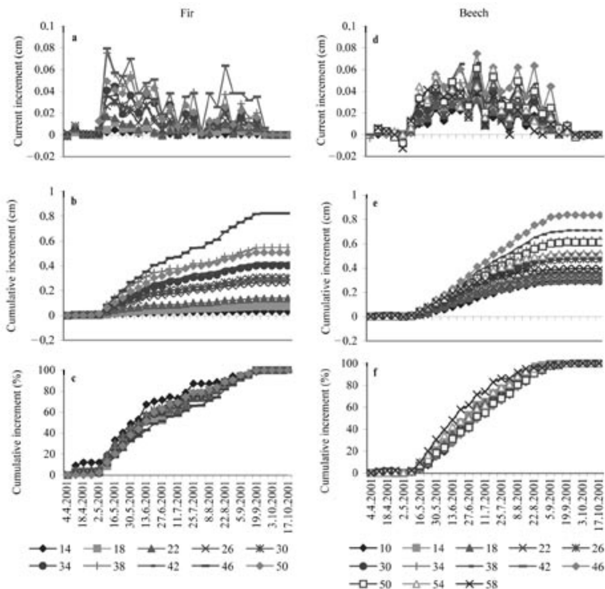
Fig. 3. Mean current (a, d) and cumulative (b, e) diameter increment of silver fir and beech in particular diameter classes and its relative expression in % (c, f) of the total annual increment
