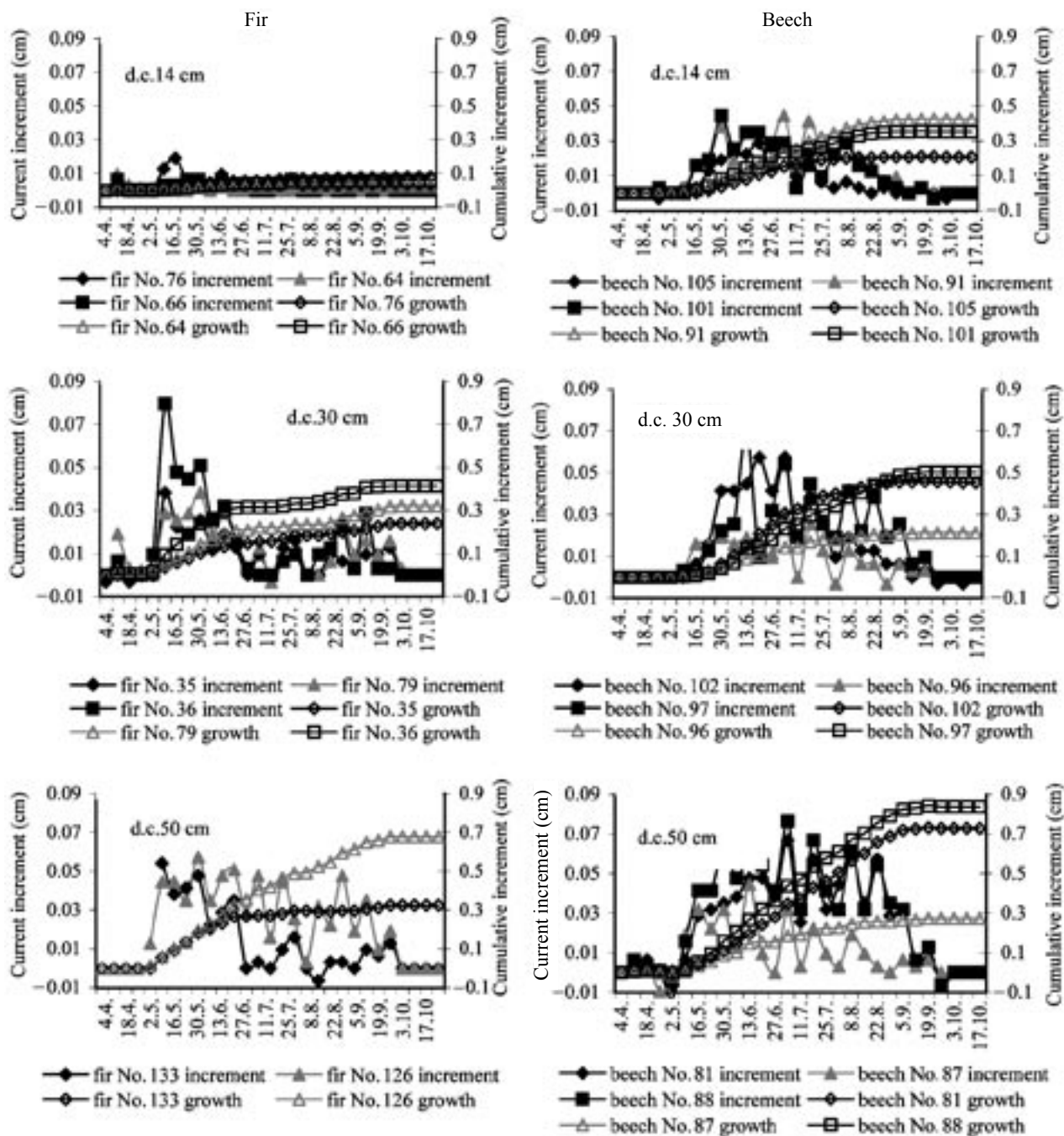
Fig. 4. Growth and increment curves of selected sample trees of silver fir and beech in diameter classes (d.c.) of 14, 30 and 50 cm
