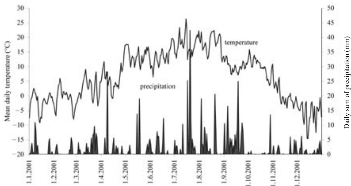
Fig. 1. Mean daily temperatures and daily precipitation totals in 2001
