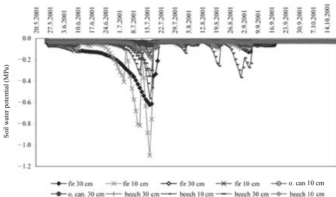
Fig. 2. The course of soil water potential below silver fir, beech and open canopy in 2001 (MPa)
