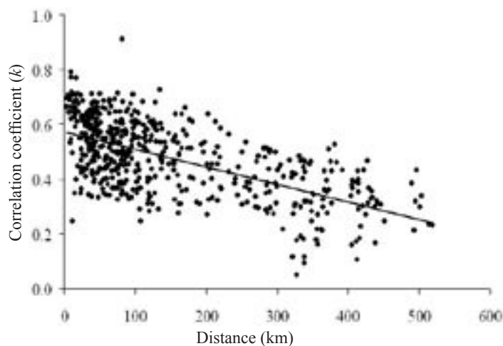
Fig. 5. Dependence between the value of the correlation coefficient ( k ) between the chronologies and the distance between the sites. The value of k = 0.3017 for the significance level ( P \leq 0.01 )
